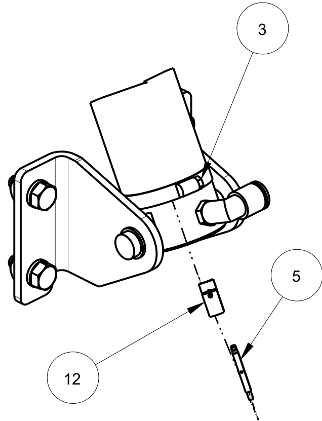
DETAIL A SCALE 1/2
